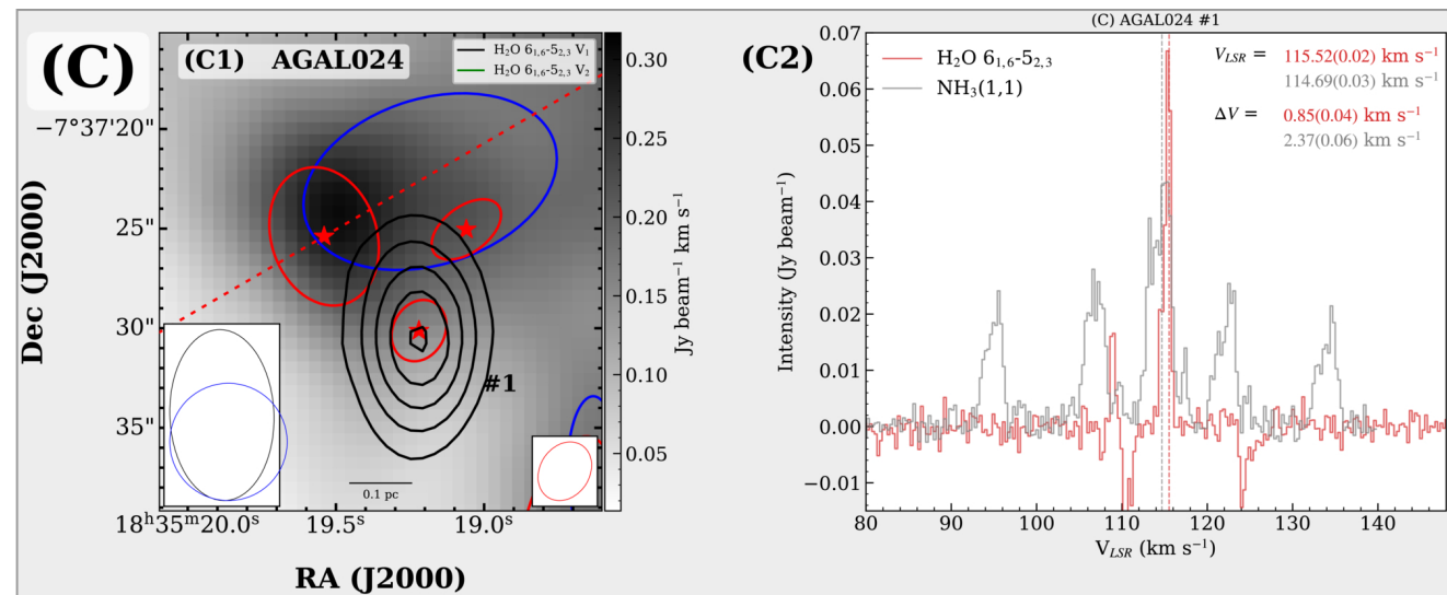
(C) The interval is 113.0–117.0 km s -1 for Reg. #1. The black contours start at 28.7 mJy beam -1 km s -1 and increase in steps of 20.5 mJy beam -1 km s -1 .
