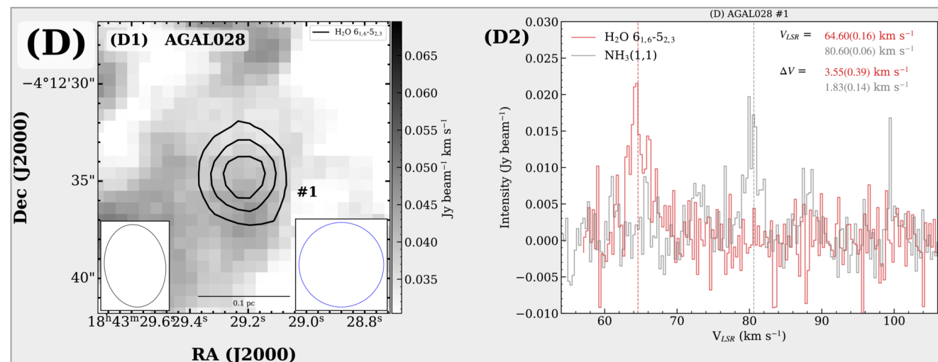
(D) The interval is 60.0–69.0 km s -1 for Reg. #1. The black contours start at 31.9 mJy beam -1 km s -1 and increase in steps of 23.9 mJy beam -1 km s -1 .
