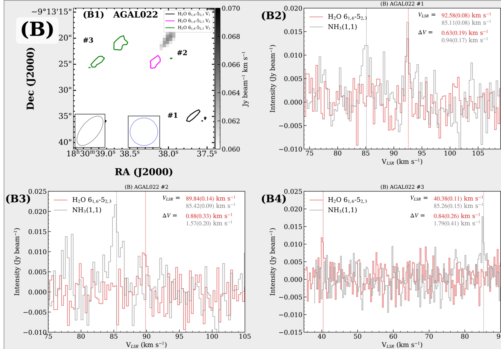
(B) The intervals are 92.0–93.2 km s -1 for Reg. #1, 89.0–90.5 km s -1 for Reg. #2, and 39.2–41.6 km s -1 for Reg. #3. The black, magenta, and green contours start at 10.3, 11.6, and 14.6 mJy beam -1 km s -1 , respectively.
