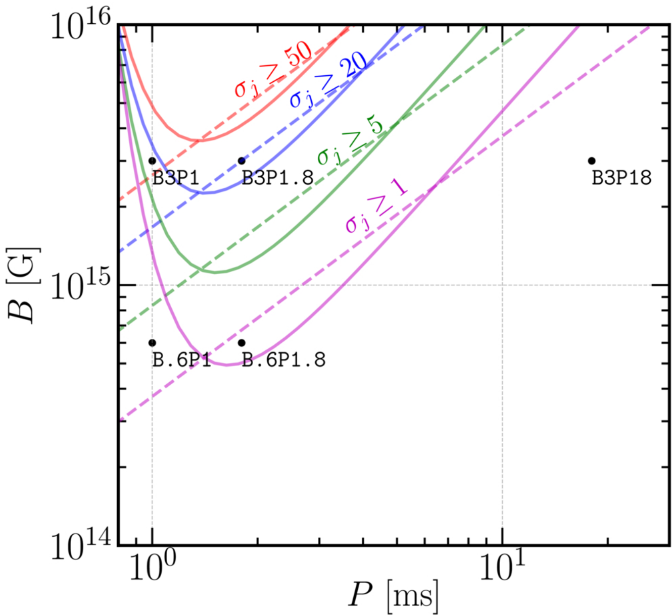
Figure B1. from Dhruv K. Desai et al 2026 Astrophys. J. Lett. 1009 doi:10.3847/2041-8213/aea3e9 https://dx.doi.org/10.3847/2041-8213/aea3e9 © 2026. The Author(s). Published by the American Astronomical Society.
