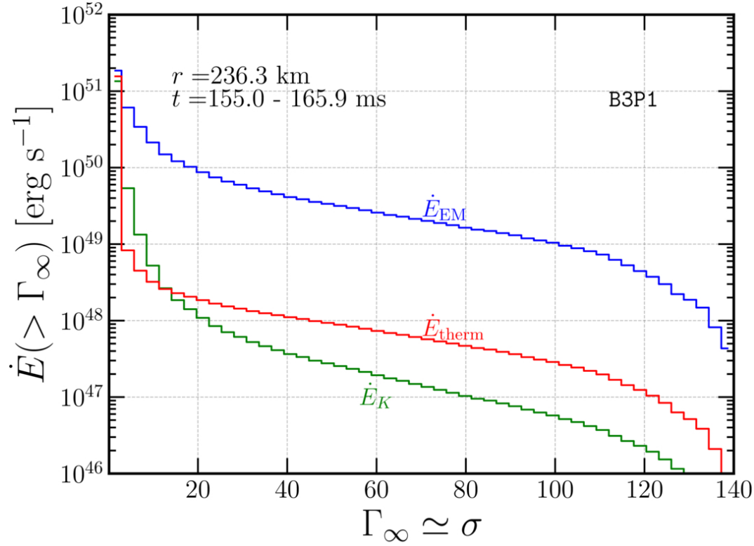
Figure 5. from Dhruv K. Desai et al 2026 Astrophys. J. Lett. 1009 doi:10.3847/2041-8213/aea3e9 https://dx.doi.org/10.3847/2041-8213/aea3e9 © 2026. The Author(s). Published by the American Astronomical Society.
