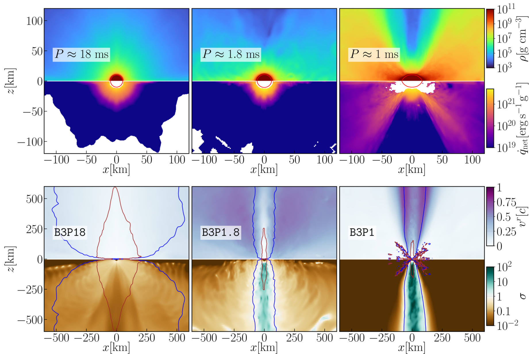
Figure 2. from Dhruv K. Desai et al 2026 Astrophys. J. Lett. 1009 doi:10.3847/2041-8213/aea3e9 https://dx.doi.org/10.3847/2041-8213/aea3e9 © 2026. The Author(s). Published by the American Astronomical Society.
