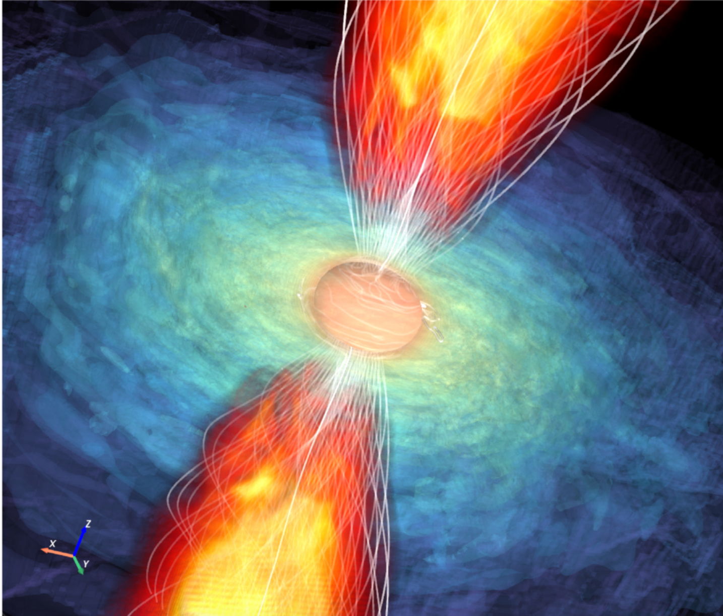
Figure 1. from Dhruv K. Desai et al 2026 Astrophys. J. Lett. 1009 doi:10.3847/2041-8213/aea3e9 https://dx.doi.org/10.3847/2041-8213/aea3e9 © 2026. The Author(s). Published by the American Astronomical Society.
