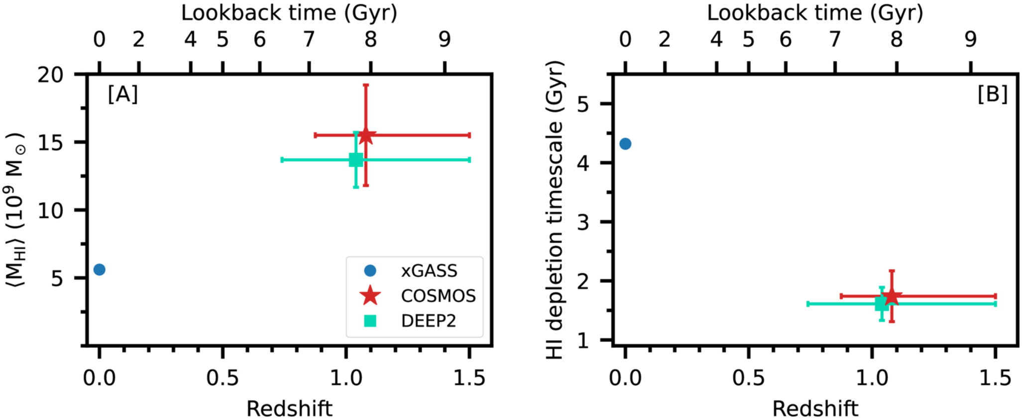
Figure 5. from Balpreet Kaur et al 2026 Astrophys. J. Lett. 1009 doi:10.3847/2041-8213/aea3e8 https://dx.doi.org/10.3847/2041-8213/aea3e8 © 2026. The Author(s). Published by the American Astronomical Society.
