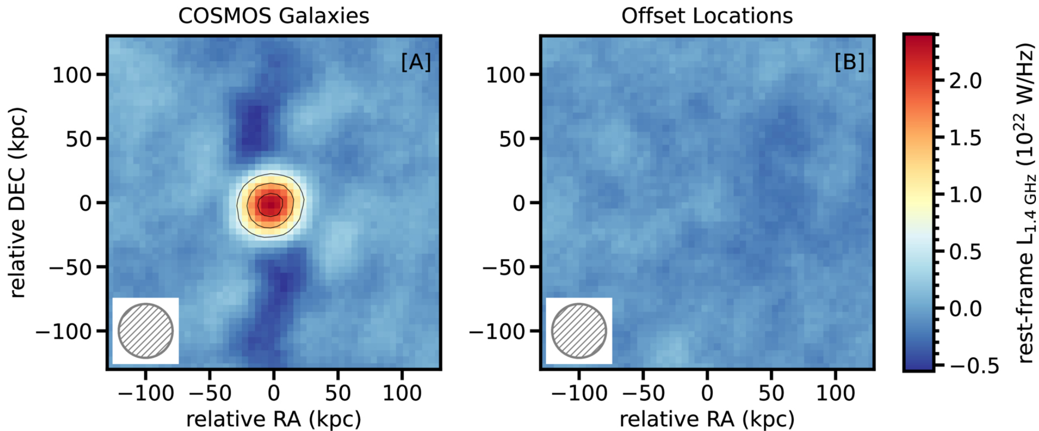
Figure 4. from Balpreet Kaur et al 2026 Astrophys. J. Lett. 1009 doi:10.3847/2041-8213/aea3e8 https://dx.doi.org/10.3847/2041-8213/aea3e8 © 2026. The Author(s). Published by the American Astronomical Society.
