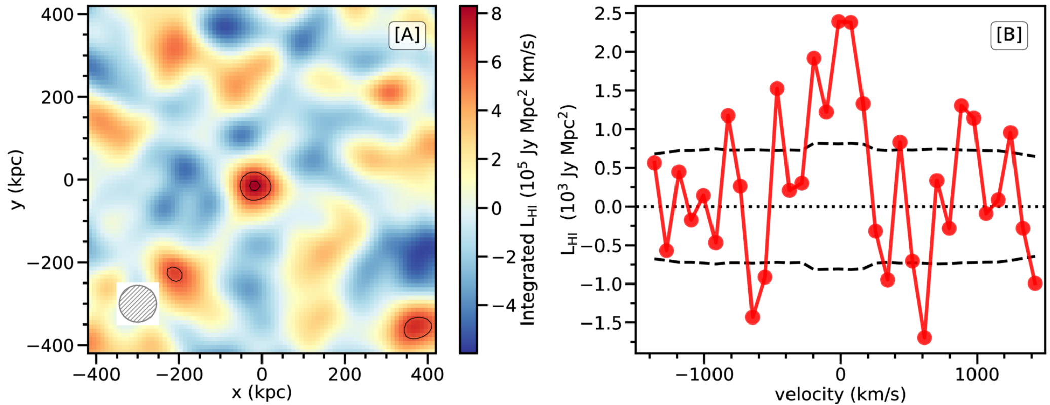
Figure 3. from Balpreet Kaur et al 2026 Astrophys. J. Lett. 1009 doi:10.3847/2041-8213/aea3e8 https://dx.doi.org/10.3847/2041-8213/aea3e8 © 2026. The Author(s). Published by the American Astronomical Society.
