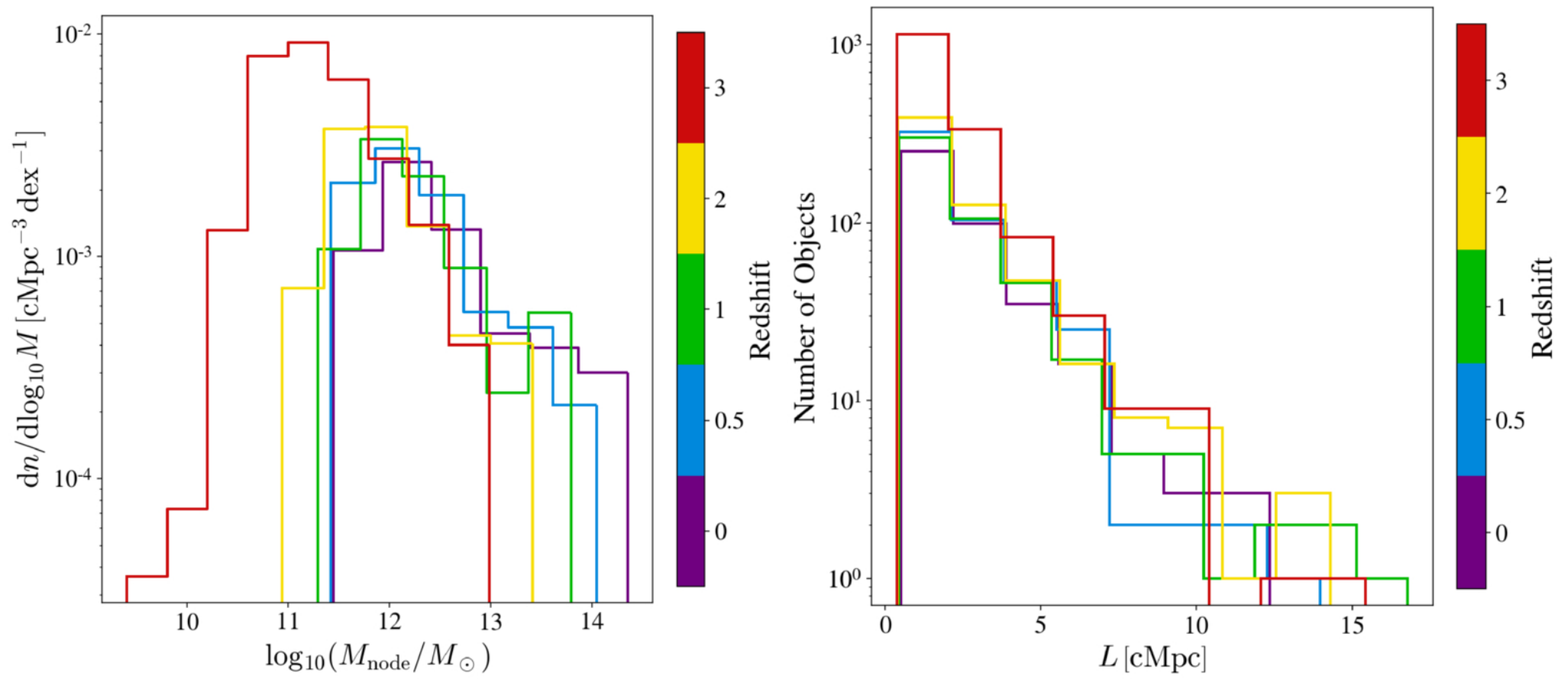
Figure A1. from Peng Xu et al 2026 Astrophys. J. Lett. 1009 doi:10.3847/2041-8213/aea298 https://dx.doi.org/10.3847/2041-8213/aea298 © 2026. The Author(s). Published by the American Astronomical Society.
