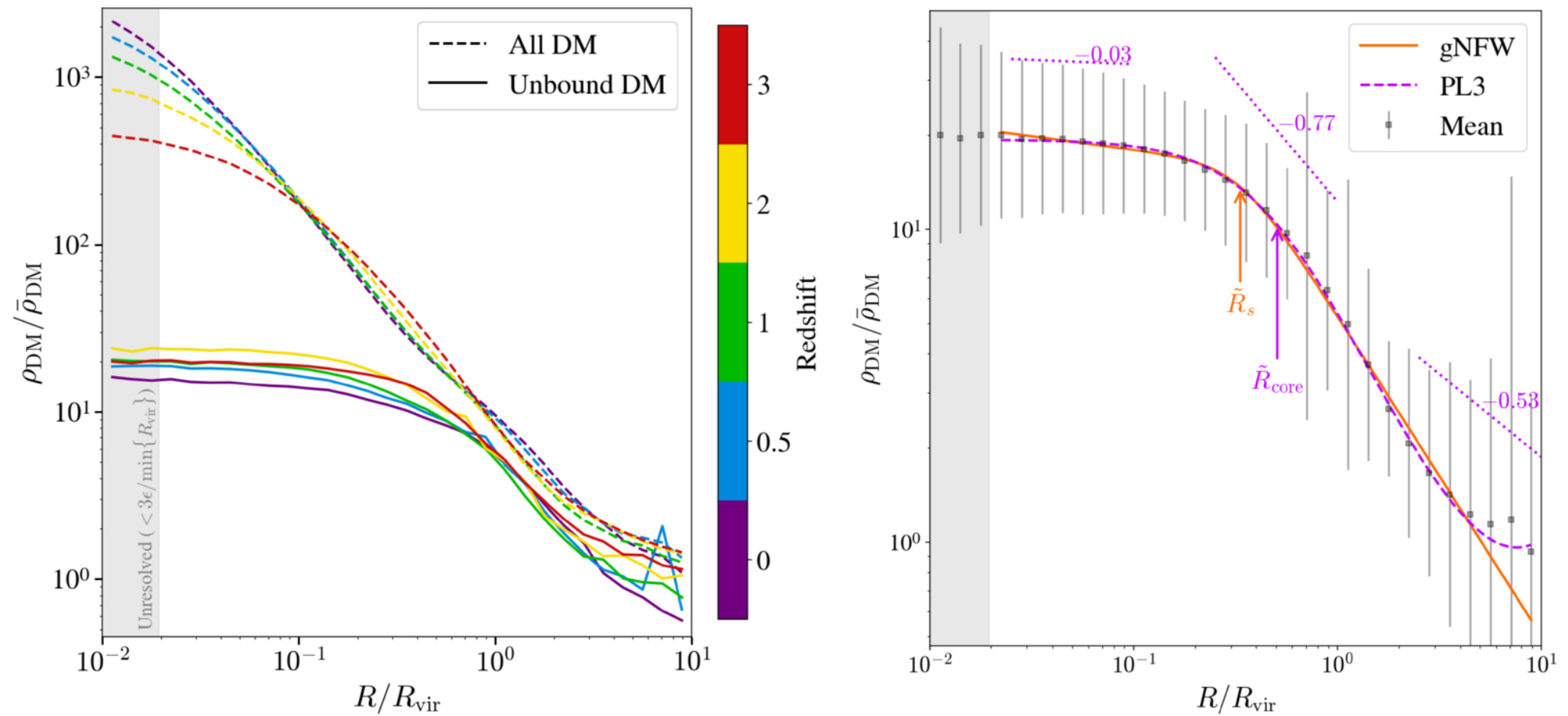
Figure 5. from Peng Xu et al 2026 Astrophys. J. Lett. 1009 doi:10.3847/2041-8213/aea298 https://dx.doi.org/10.3847/2041-8213/aea298 © 2026. The Author(s). Published by the American Astronomical Society.
