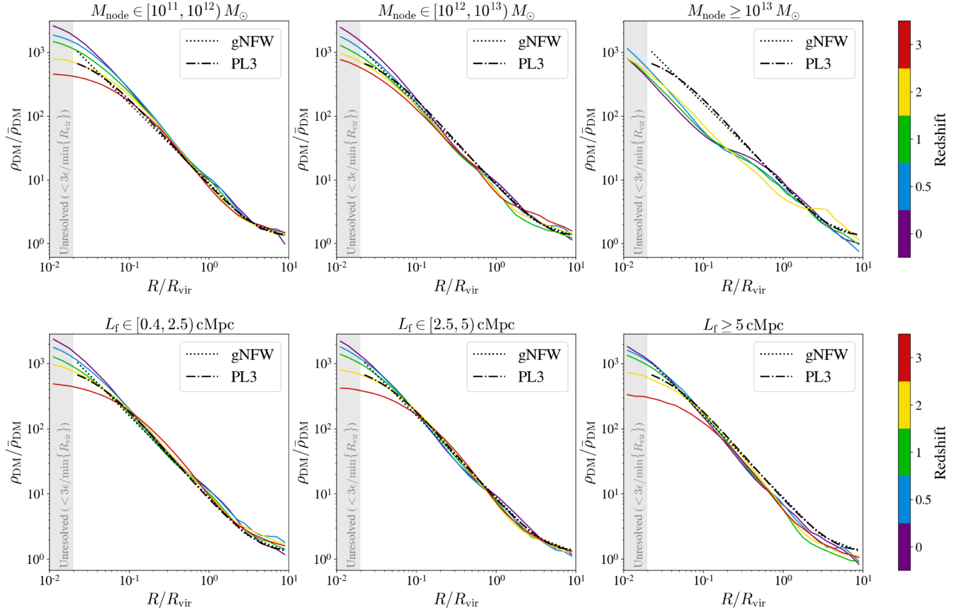
Figure 4. from Peng Xu et al 2026 Astrophys. J. Lett. 1009 doi:10.3847/2041-8213/aea298 https://dx.doi.org/10.3847/2041-8213/aea298 © 2026. The Author(s). Published by the American Astronomical Society.
