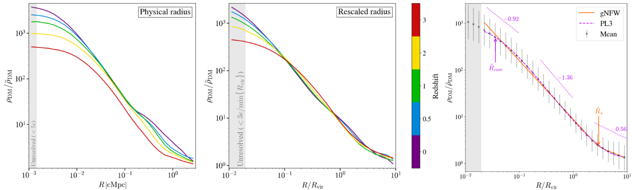
Figure 3. from Peng Xu et al 2026 Astrophys. J. Lett. 1009 doi:10.3847/2041-8213/aea298 https://dx.doi.org/10.3847/2041-8213/aea298 © 2026. The Author(s). Published by the American Astronomical Society.
