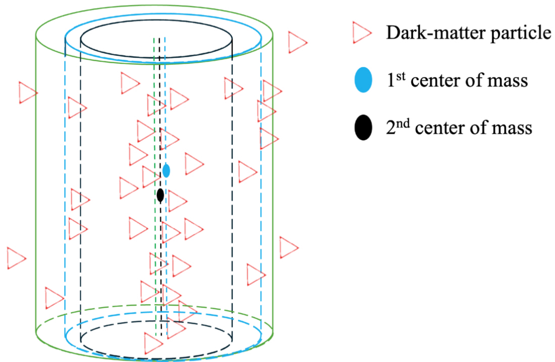
Figure 2. from Peng Xu et al 2026 Astrophys. J. Lett. 1009 doi:10.3847/2041-8213/aea298 https://dx.doi.org/10.3847/2041-8213/aea298 © 2026. The Author(s). Published by the American Astronomical Society.
