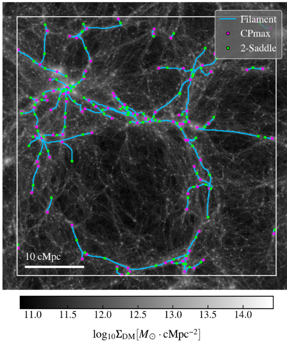
Figure 1. from Peng Xu et al 2026 Astrophys. J. Lett. 1009 doi:10.3847/2041-8213/aea298 https://dx.doi.org/10.3847/2041-8213/aea298 © 2026. The Author(s). Published by the American Astronomical Society.
