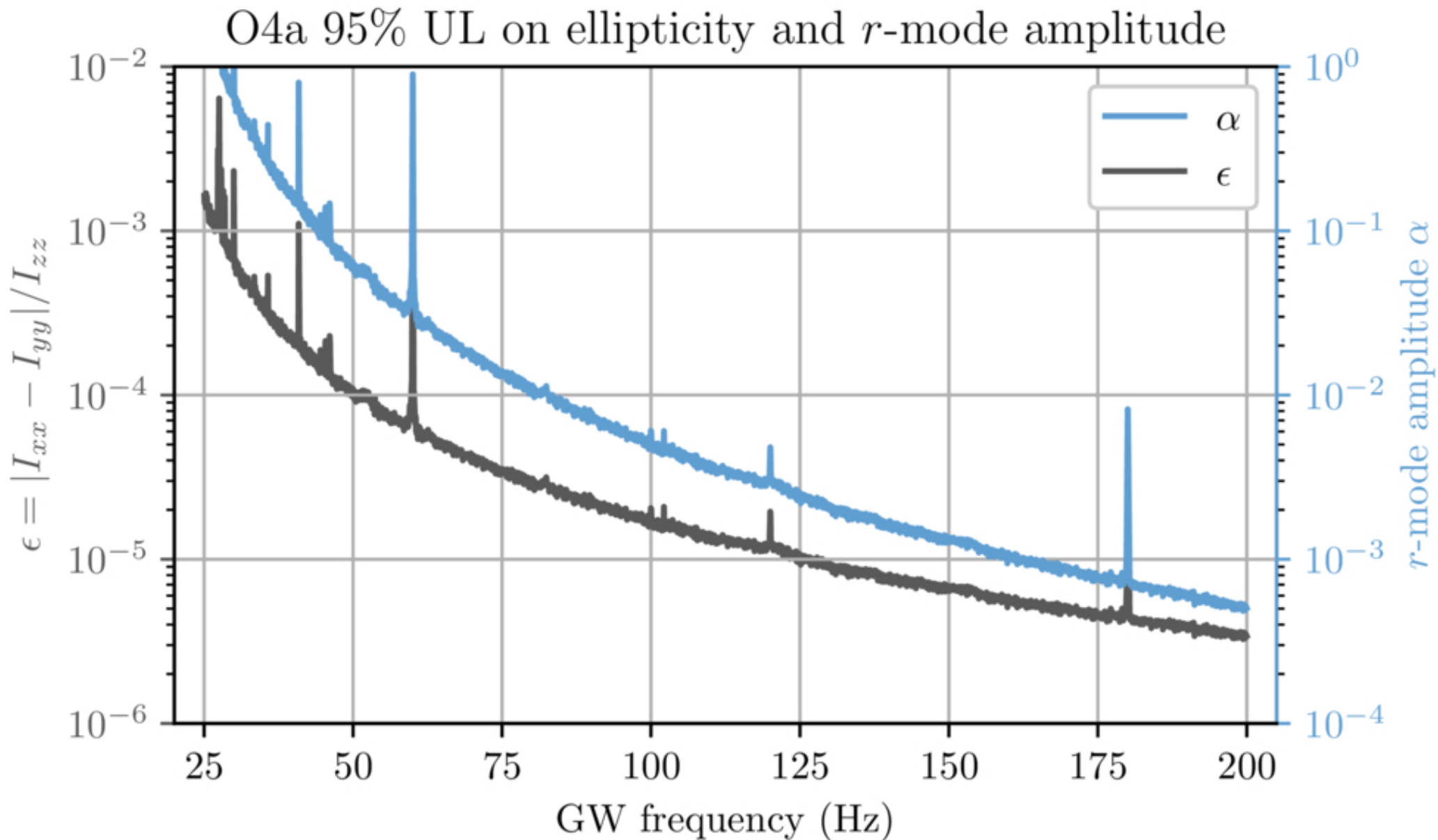
Figure 7. from A. G. Abac et al 2026 Astrophys. J. Lett. 1010 doi:10.3847/2041-8213/aea296 https://dx.doi.org/10.3847/2041-8213/aea296 © 2026. The Author(s). Published by the American Astronomical Society.
