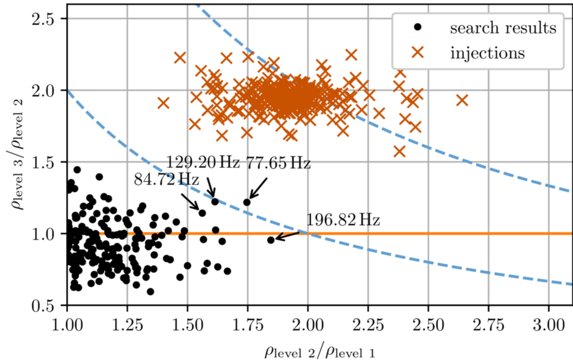
Figure 4. from A. G. Abac et al 2026 Astrophys. J. Lett. 1010 doi:10.3847/2041-8213/aea296 https://dx.doi.org/10.3847/2041-8213/aea296 © 2026. The Author(s). Published by the American Astronomical Society.
