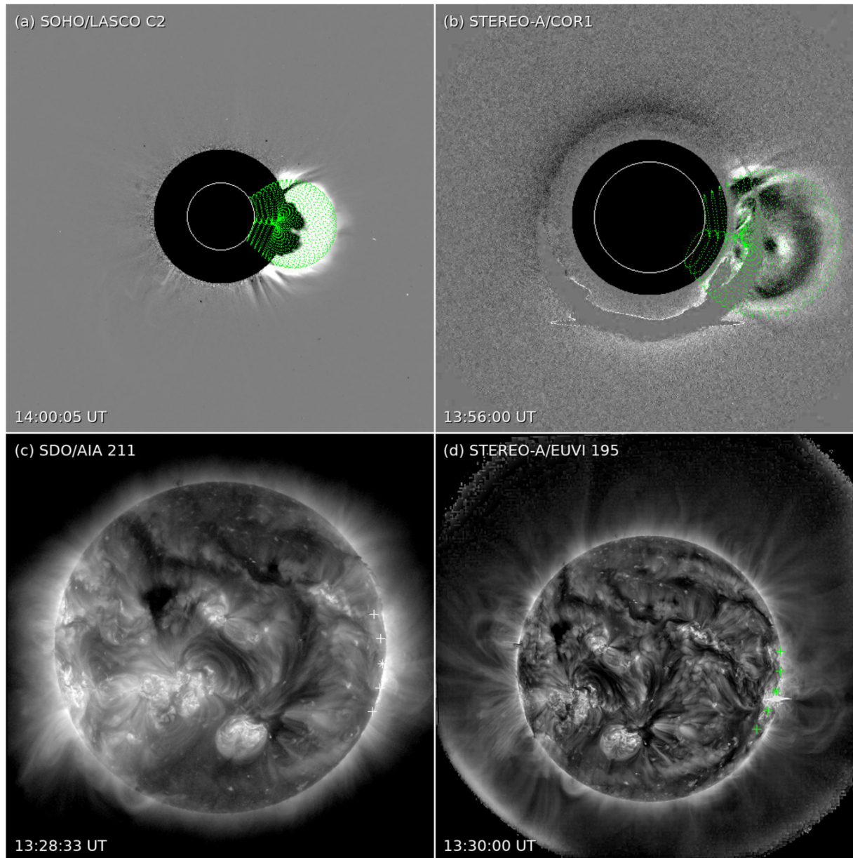
Figure B1. from Saurabh Tripathi et al 2026 Astrophys. J. Lett. 1009 doi:10.3847/2041-8213/aea295 https://dx.doi.org/10.3847/2041-8213/aea295 © 2026. The Author(s). Published by the American Astronomical Society.
