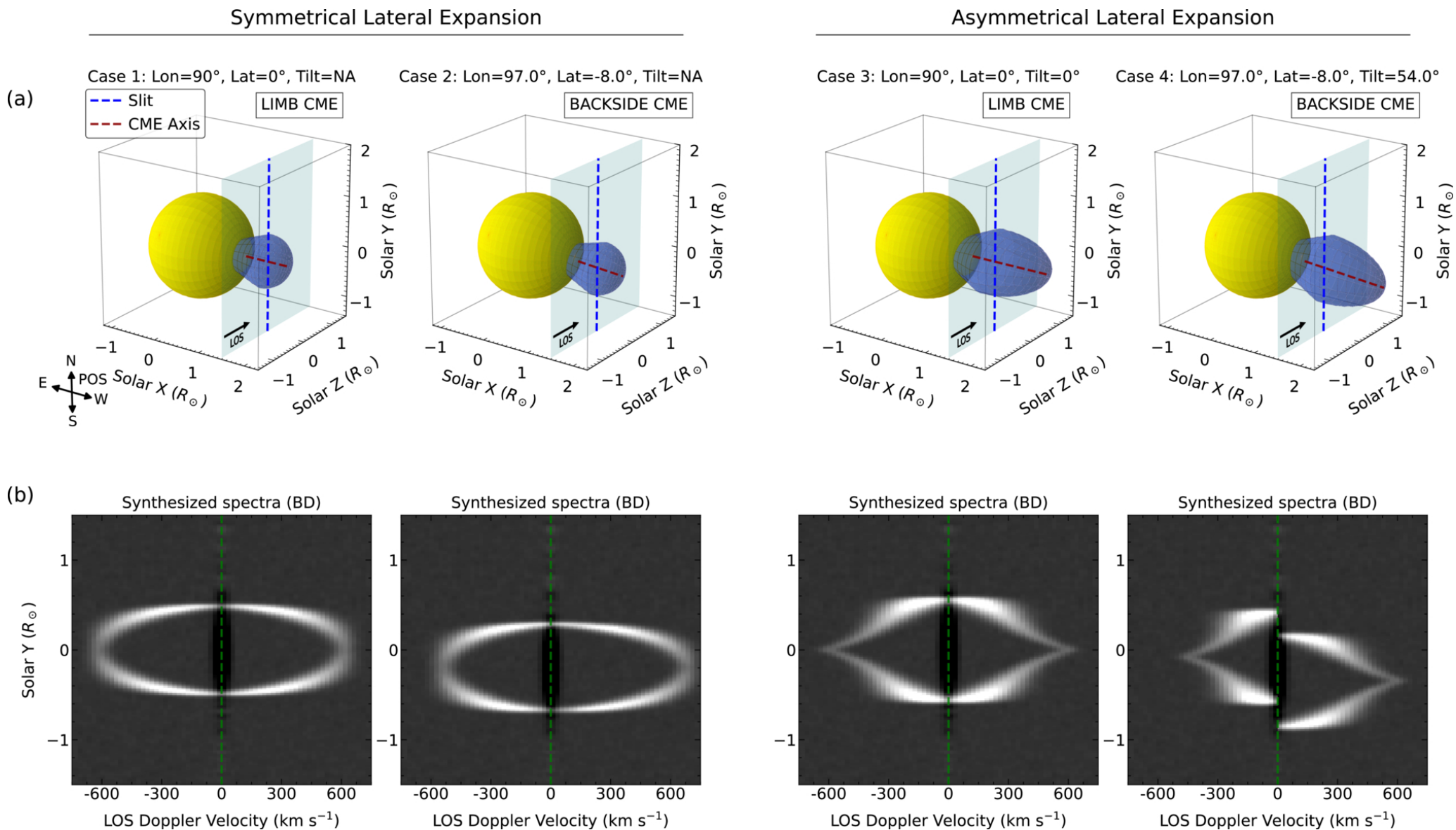
Figure 5. from Saurabh Tripathi et al 2026 Astrophys. J. Lett. 1009 doi:10.3847/2041-8213/aea295 https://dx.doi.org/10.3847/2041-8213/aea295 © 2026. The Author(s). Published by the American Astronomical Society.
