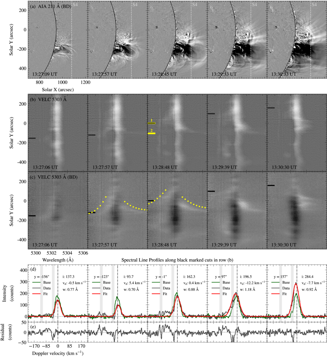
Figure 2. from Saurabh Tripathi et al 2026 Astrophys. J. Lett. 1009 doi:10.3847/2041-8213/aea295 https://dx.doi.org/10.3847/2041-8213/aea295 © 2026. The Author(s). Published by the American Astronomical Society.
