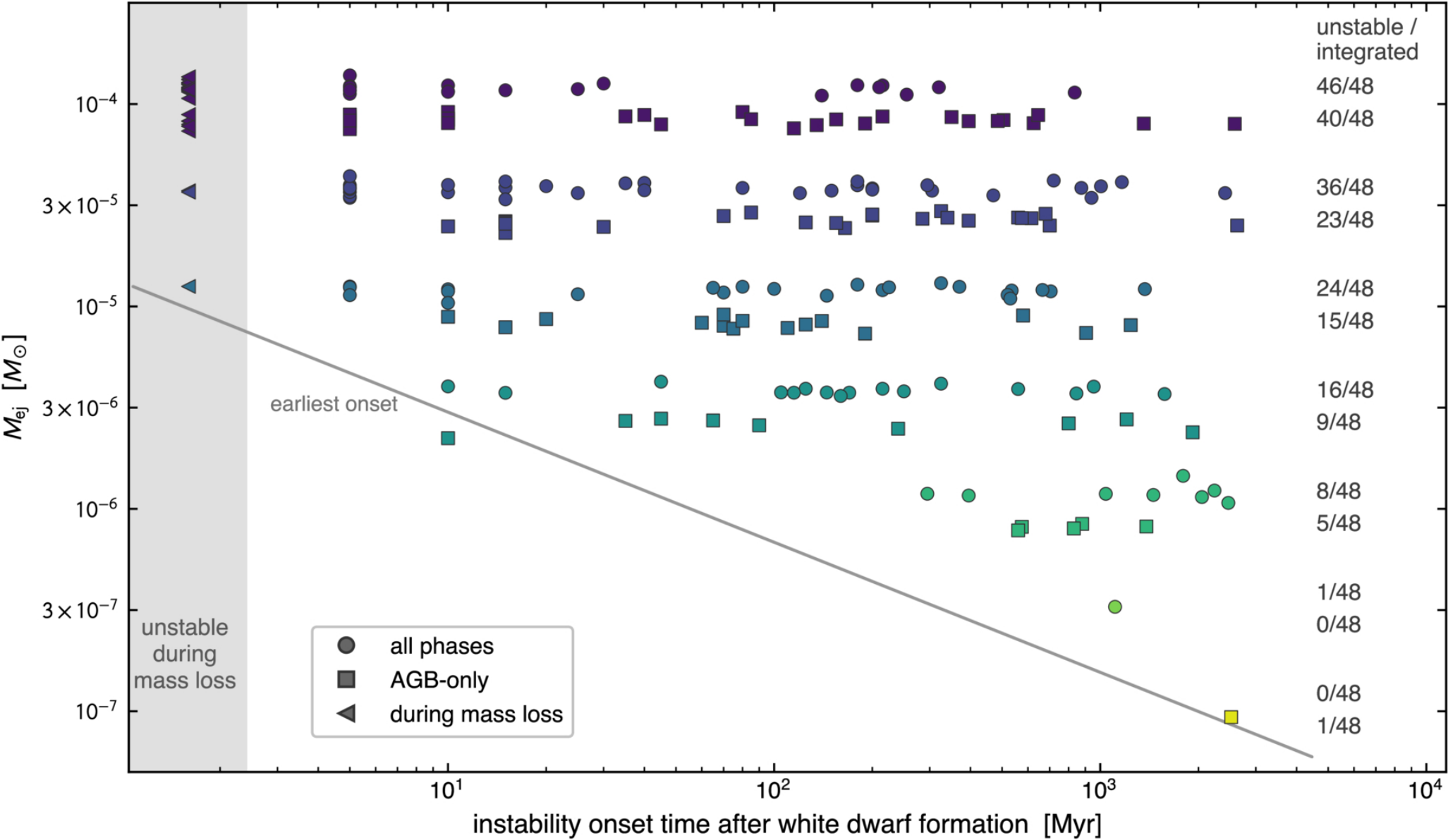
Figure B1. from Konstantin Batygin et al 2026 Astrophys. J. Lett. 1009 doi:10.3847/2041-8213/aea290 https://dx.doi.org/10.3847/2041-8213/aea290 © 2026. The Author(s). Published by the American Astronomical Society.
