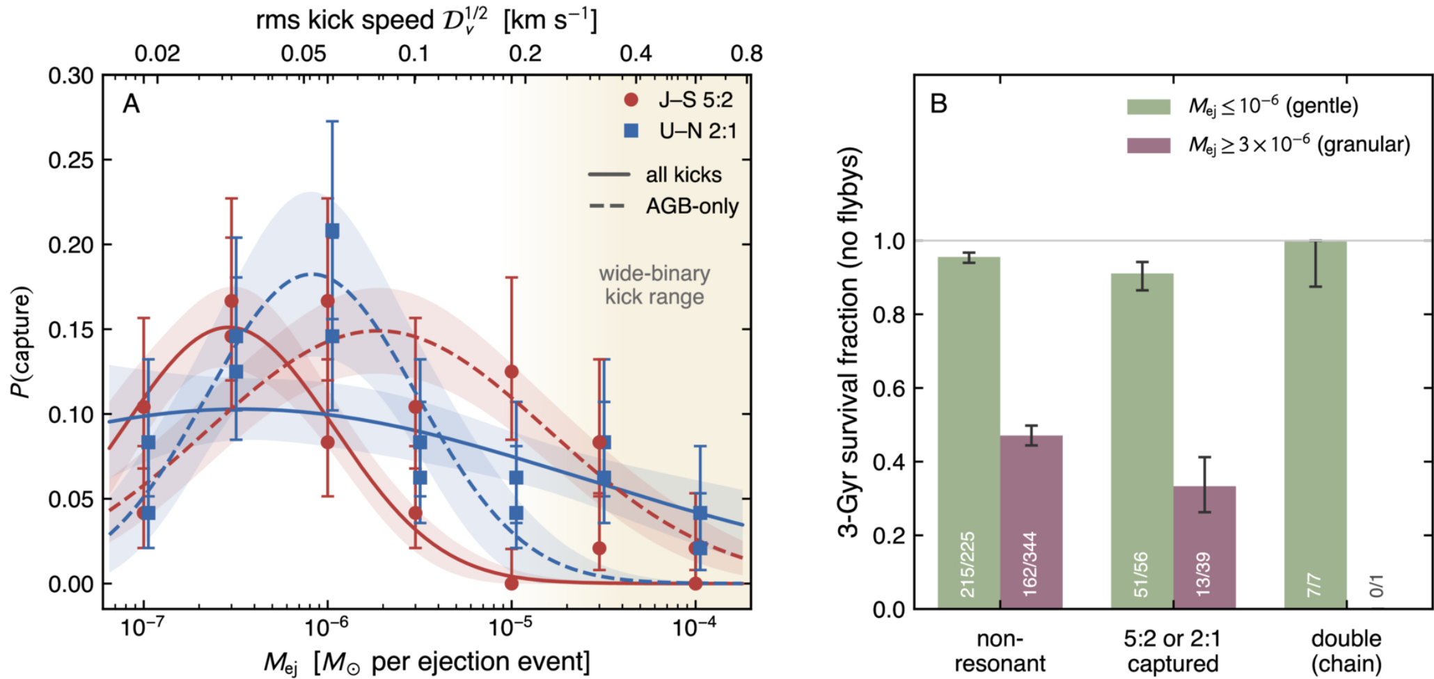
Figure 5. from Konstantin Batygin et al 2026 Astrophys. J. Lett. 1009 doi:10.3847/2041-8213/aea290 https://dx.doi.org/10.3847/2041-8213/aea290 © 2026. The Author(s). Published by the American Astronomical Society.
