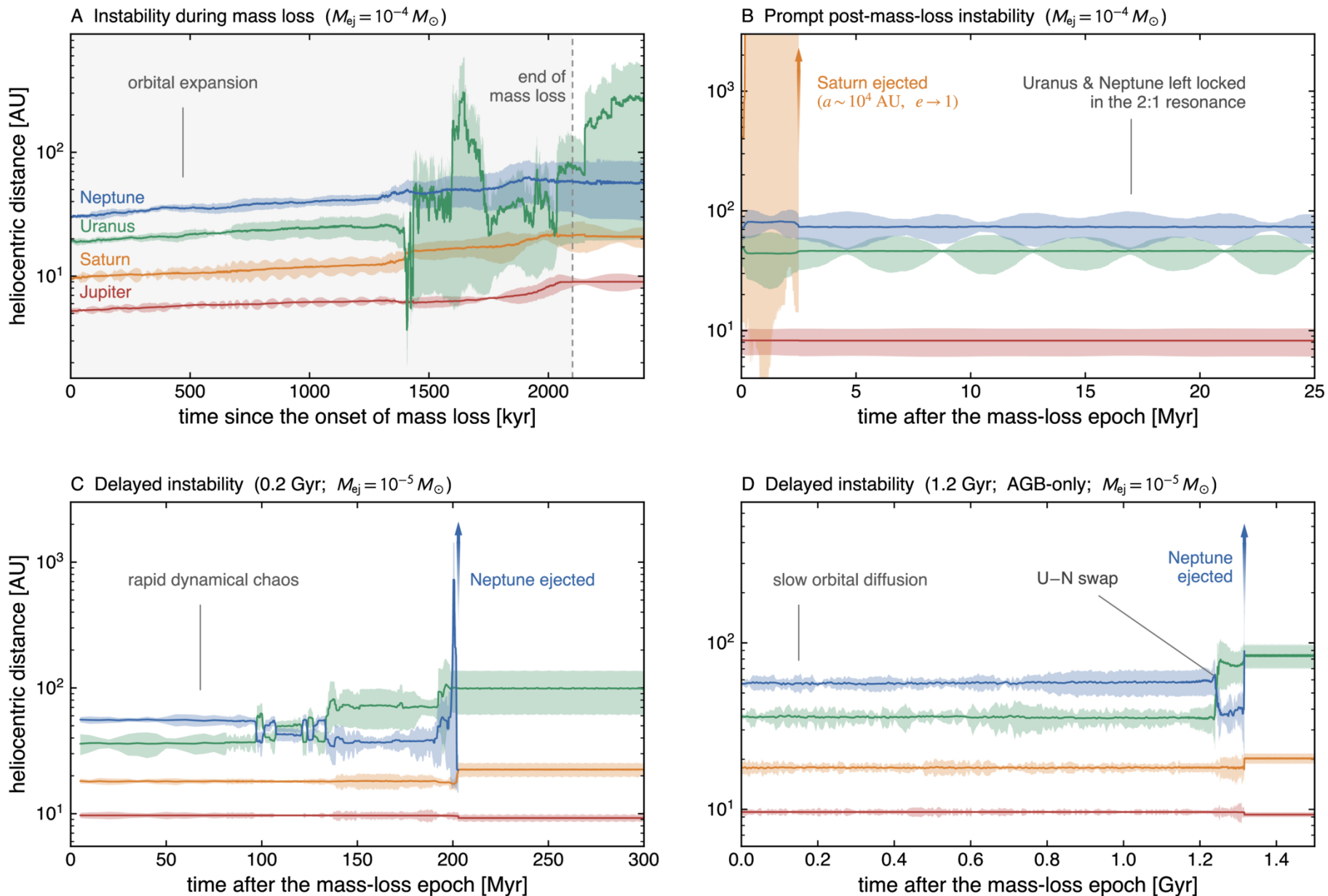
Figure 3. from Konstantin Batygin et al 2026 Astrophys. J. Lett. 1009 doi:10.3847/2041-8213/aea290 https://dx.doi.org/10.3847/2041-8213/aea290 © 2026. The Author(s). Published by the American Astronomical Society.
