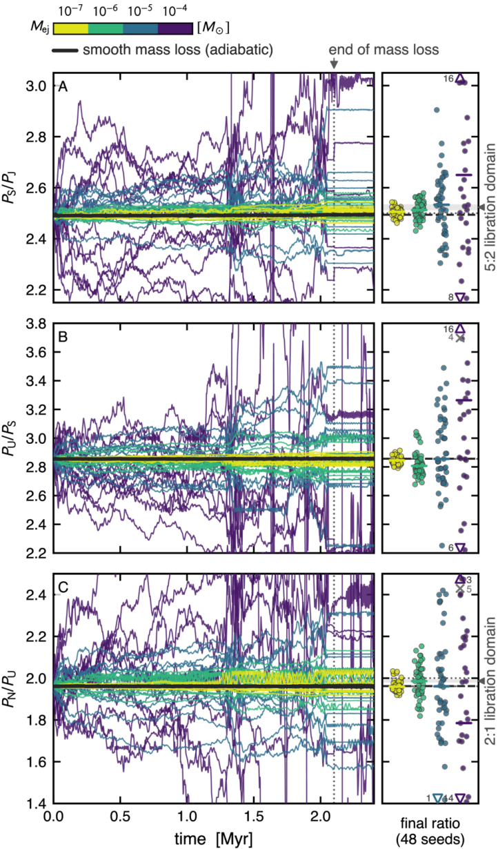
Figure 1. from Konstantin Batygin et al 2026 Astrophys. J. Lett. 1009 doi:10.3847/2041-8213/aea290 https://dx.doi.org/10.3847/2041-8213/aea290 © 2026. The Author(s). Published by the American Astronomical Society.
