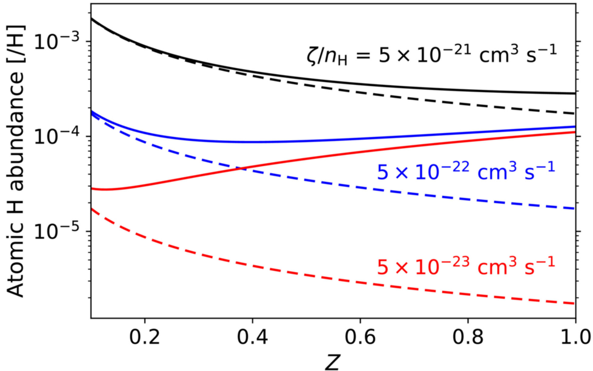
Figure A1. from Kenji Furuya et al 2026 Astrophys. J. Lett. 1009 doi:10.3847/2041-8213/aea221 https://dx.doi.org/10.3847/2041-8213/aea221 © 2026. The Author(s). Published by the American Astronomical Society.
