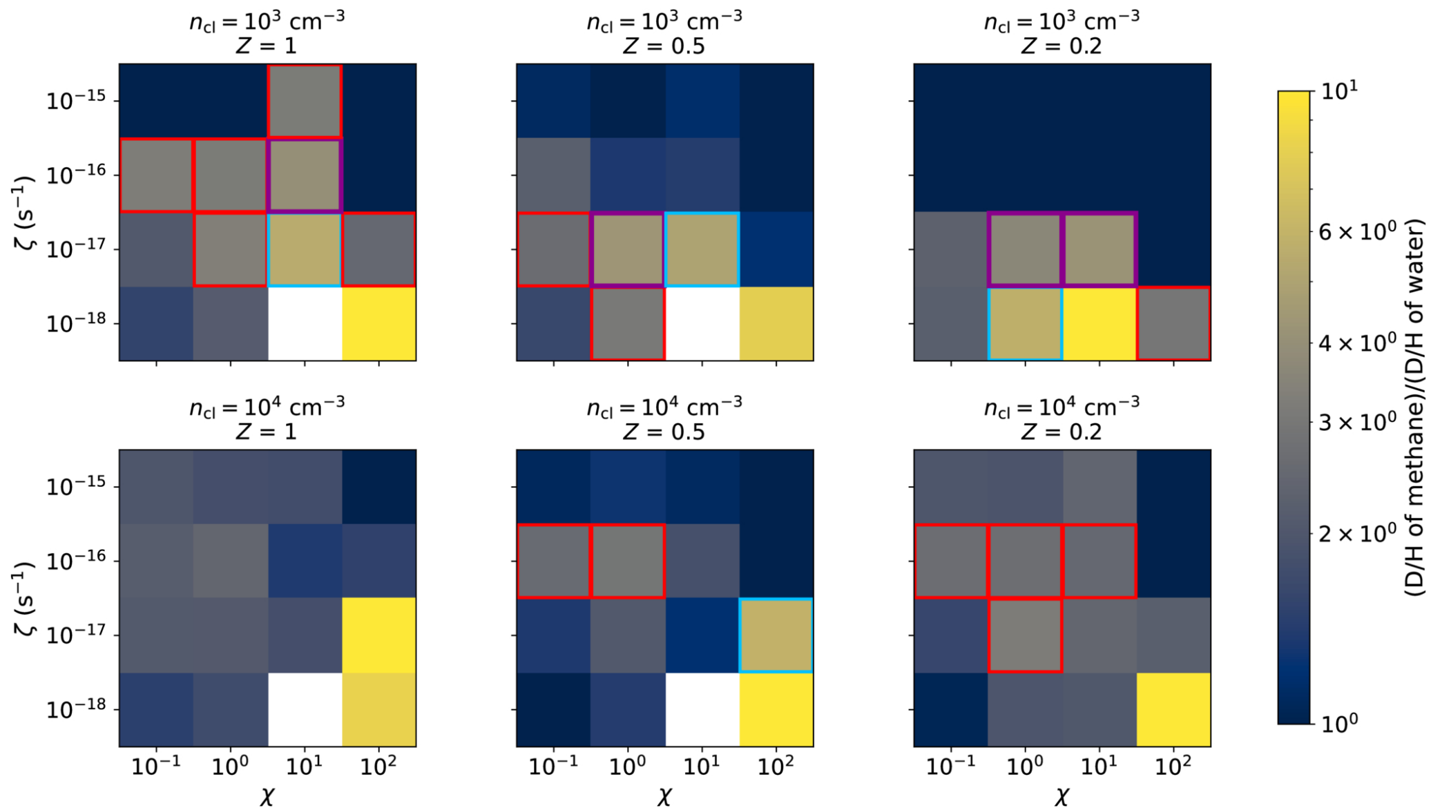
Figure 3. from Kenji Furuya et al 2026 Astrophys. J. Lett. 1009 doi:10.3847/2041-8213/aea221 https://dx.doi.org/10.3847/2041-8213/aea221 © 2026. The Author(s). Published by the American Astronomical Society.
