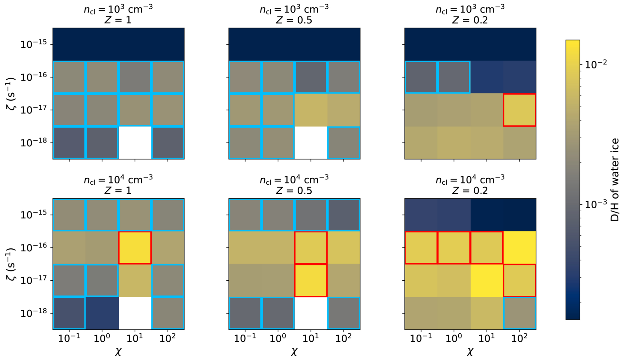
Figure 2. from Kenji Furuya et al 2026 Astrophys. J. Lett. 1009 doi:10.3847/2041-8213/aea221 https://dx.doi.org/10.3847/2041-8213/aea221 © 2026. The Author(s). Published by the American Astronomical Society.
