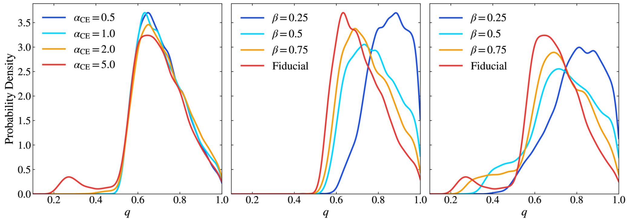
Figure 5. from Rui-Chong Hu et al 2026 Astrophys. J. Lett. 1009 doi:10.3847/2041-8213/aea21b https://dx.doi.org/10.3847/2041-8213/aea21b © 2026. The Author(s). Published by the American Astronomical Society.
