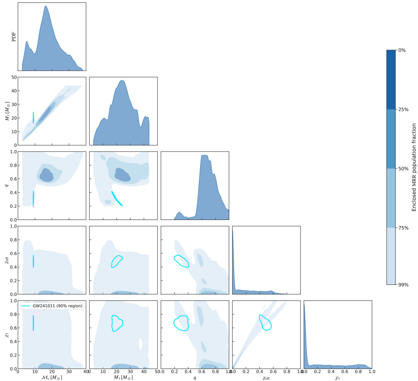
Figure 2. from Rui-Chong Hu et al 2026 Astrophys. J. Lett. 1009 doi:10.3847/2041-8213/aea21b https://dx.doi.org/10.3847/2041-8213/aea21b © 2026. The Author(s). Published by the American Astronomical Society.
