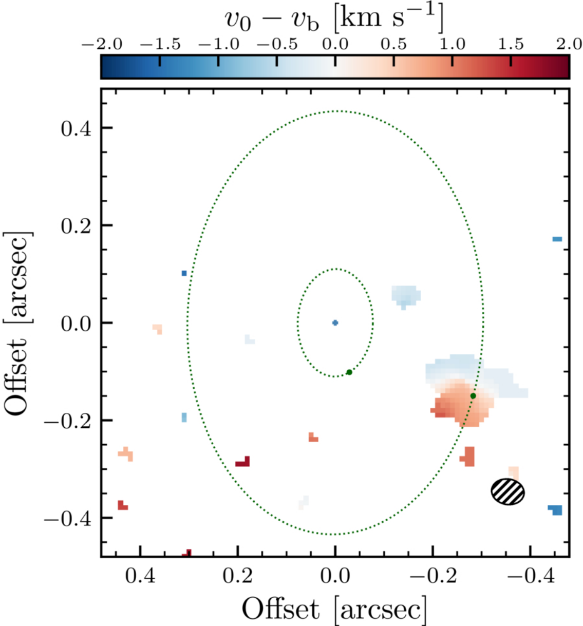
Figure 9. from Myriam Benisty et al 2026 Astrophys. J. Lett. 1009 doi:10.3847/2041-8213/aea214 https://dx.doi.org/10.3847/2041-8213/aea214 © 2026. The Author(s). Published by the American Astronomical Society.
