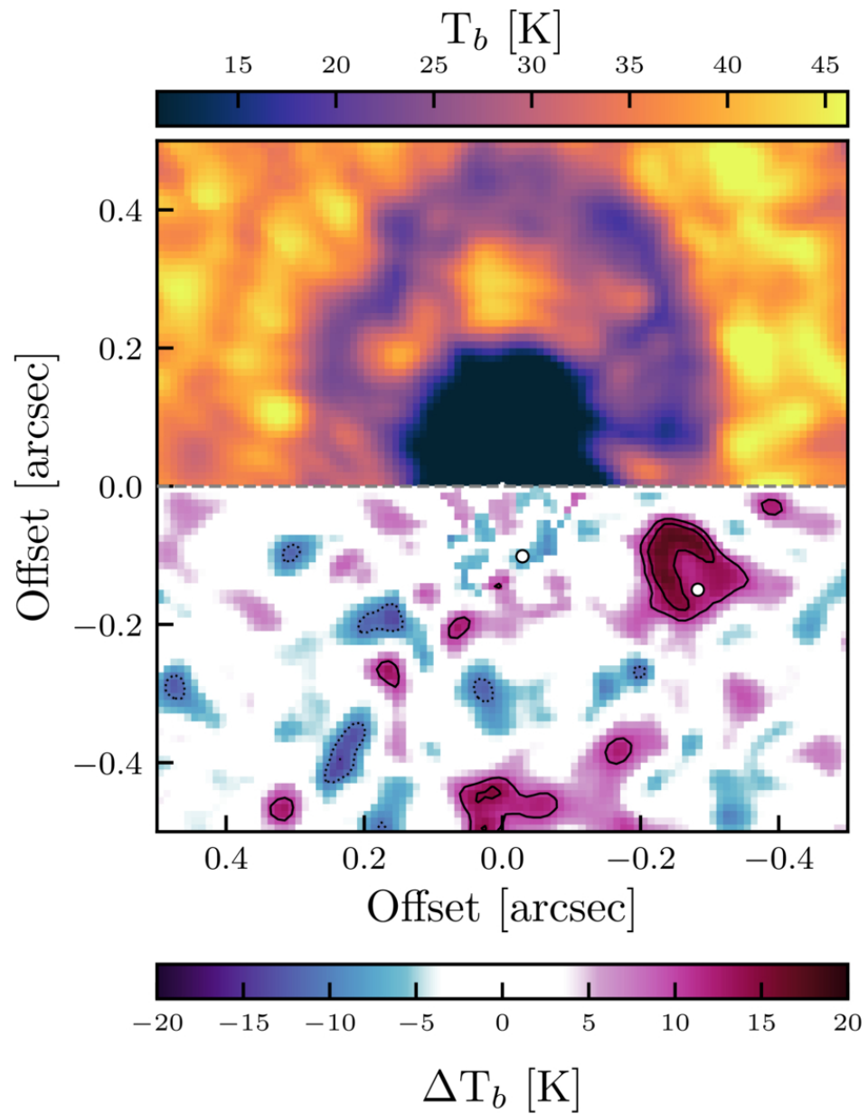
Figure 8. from Myriam Benisty et al 2026 Astrophys. J. Lett. 1009 doi:10.3847/2041-8213/aea214 https://dx.doi.org/10.3847/2041-8213/aea214 © 2026. The Author(s). Published by the American Astronomical Society.
