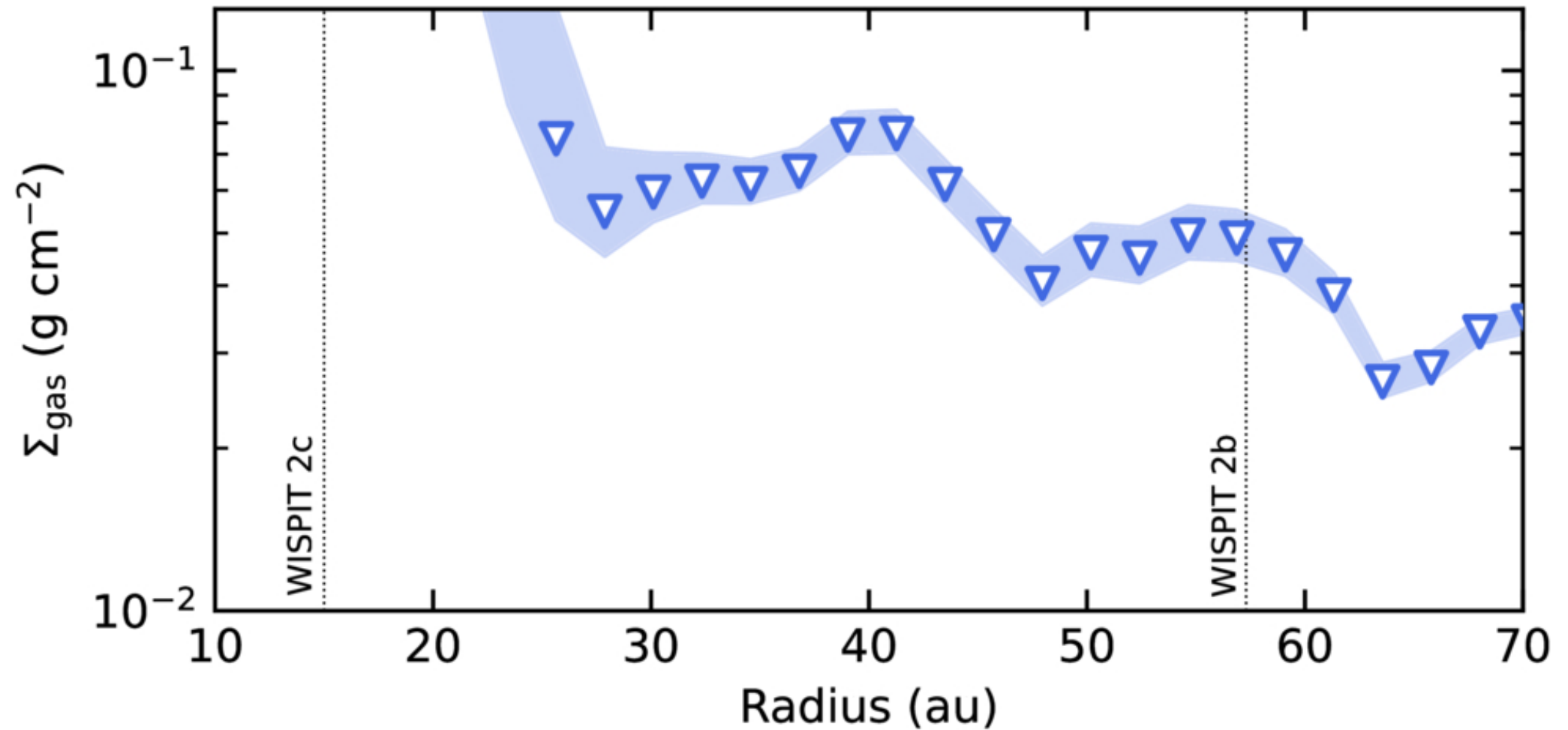
Figure 7. from Myriam Benisty et al 2026 Astrophys. J. Lett. 1009 doi:10.3847/2041-8213/aea214 https://dx.doi.org/10.3847/2041-8213/aea214 © 2026. The Author(s). Published by the American Astronomical Society.
