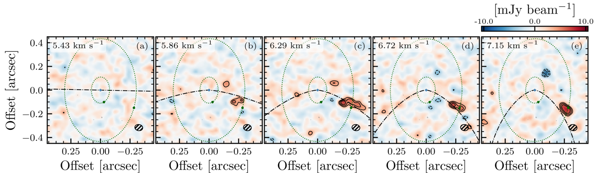
Figure 6. from Myriam Benisty et al 2026 Astrophys. J. Lett. 1009 doi:10.3847/2041-8213/aea214 https://dx.doi.org/10.3847/2041-8213/aea214 © 2026. The Author(s). Published by the American Astronomical Society.
