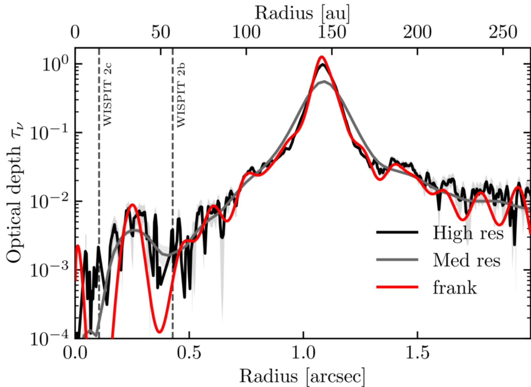
Figure 3. from Myriam Benisty et al 2026 Astrophys. J. Lett. 1009 doi:10.3847/2041-8213/aea214 https://dx.doi.org/10.3847/2041-8213/aea214 © 2026. The Author(s). Published by the American Astronomical Society.
