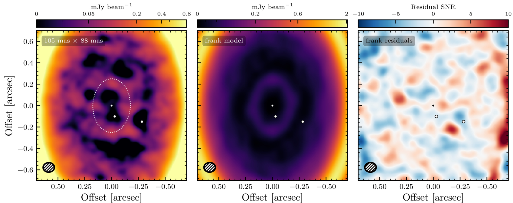
Figure 2. from Myriam Benisty et al 2026 Astrophys. J. Lett. 1009 doi:10.3847/2041-8213/aea214 https://dx.doi.org/10.3847/2041-8213/aea214 © 2026. The Author(s). Published by the American Astronomical Society.
