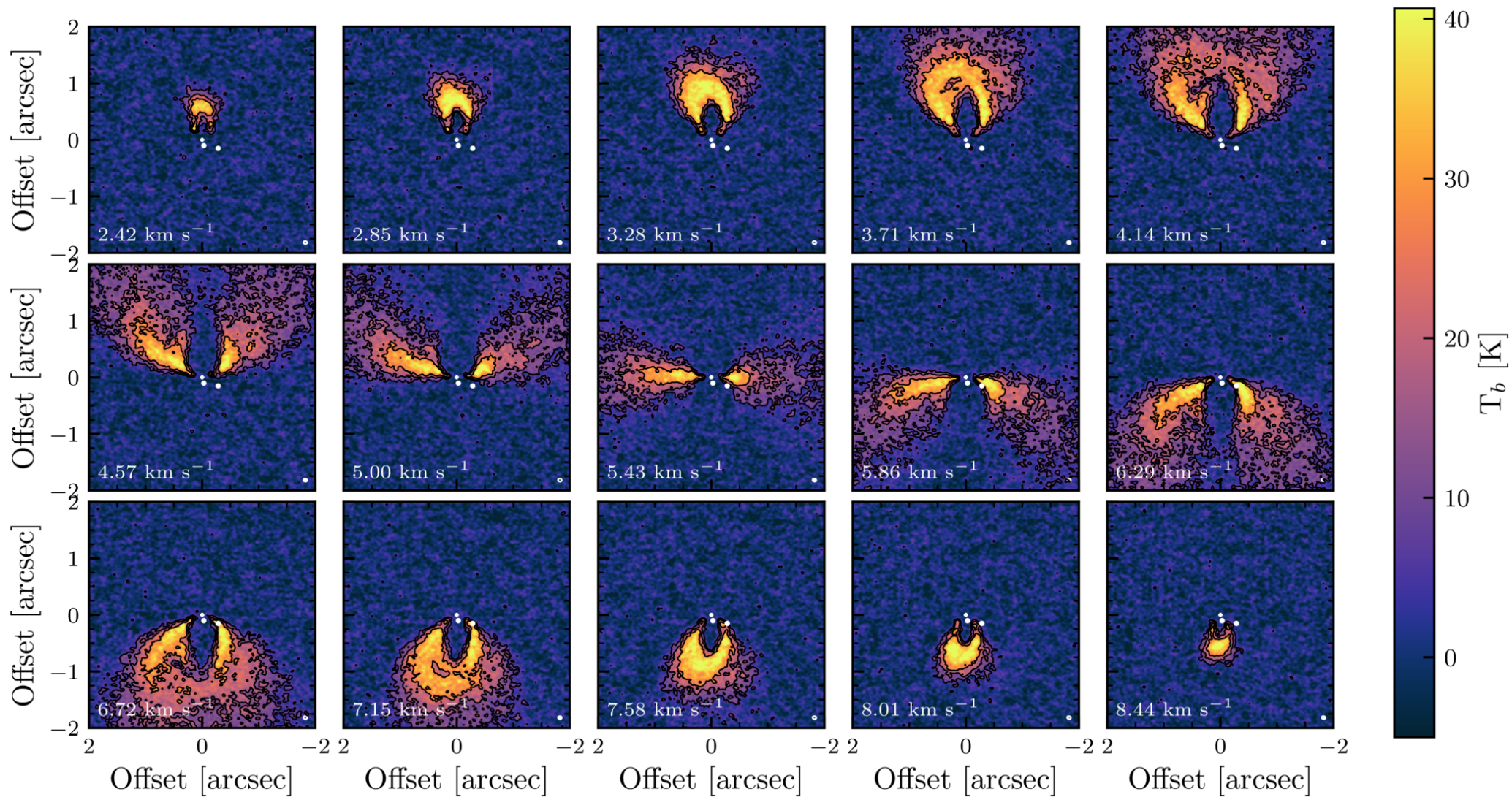
Figure F5. from Myriam Benisty et al 2026 Astrophys. J. Lett. 1009 doi:10.3847/2041-8213/aea214 https://dx.doi.org/10.3847/2041-8213/aea214 © 2026. The Author(s). Published by the American Astronomical Society.
