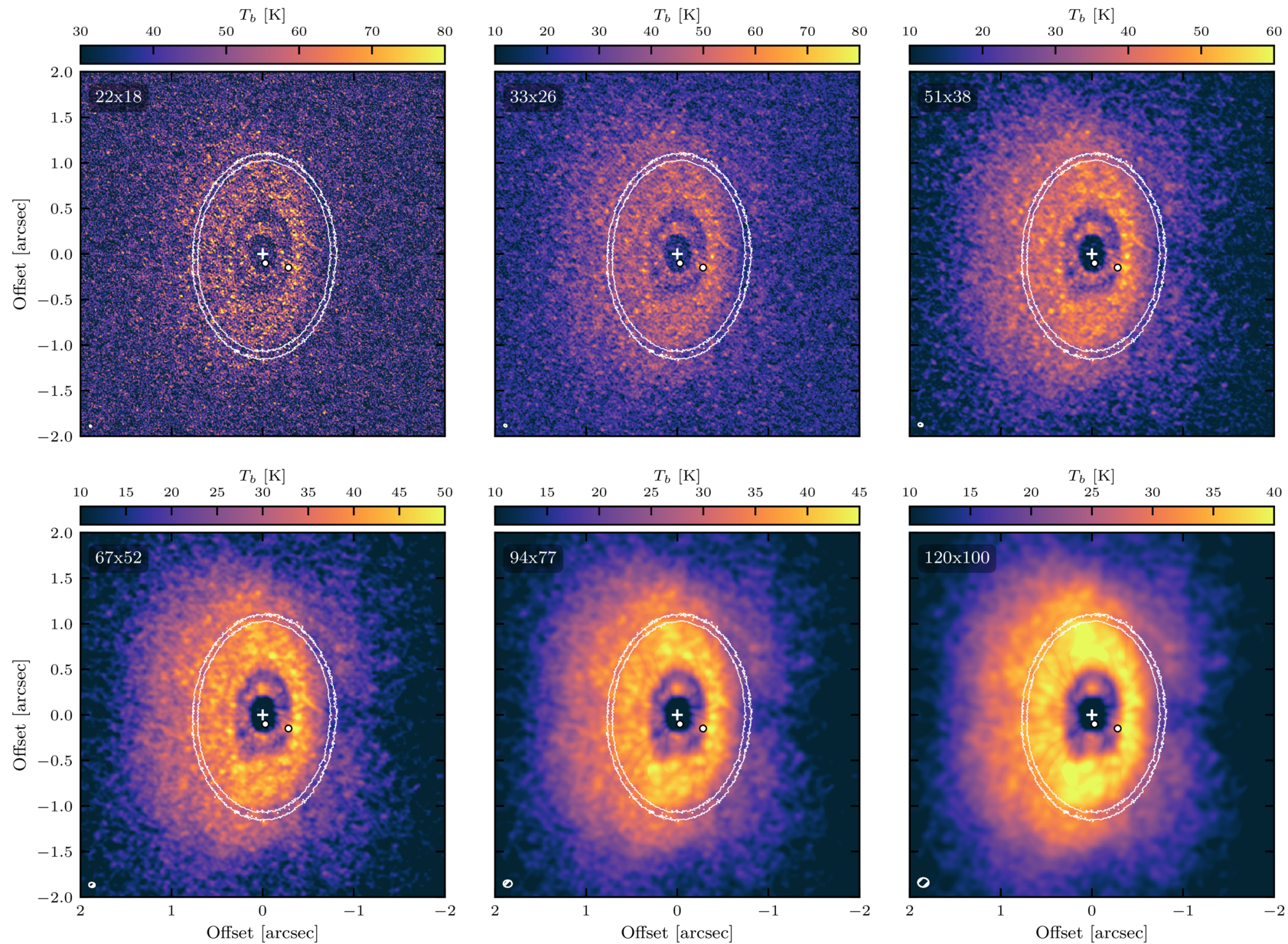
Figure F2. from Myriam Benisty et al 2026 Astrophys. J. Lett. 1009 doi:10.3847/2041-8213/aea214 https://dx.doi.org/10.3847/2041-8213/aea214 © 2026. The Author(s). Published by the American Astronomical Society.
