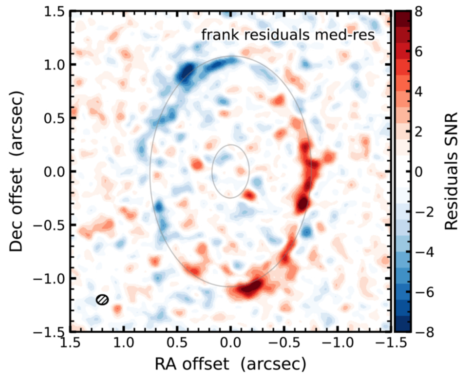
Figure F1. from Myriam Benisty et al 2026 Astrophys. J. Lett. 1009 doi:10.3847/2041-8213/aea214 https://dx.doi.org/10.3847/2041-8213/aea214 © 2026. The Author(s). Published by the American Astronomical Society.
