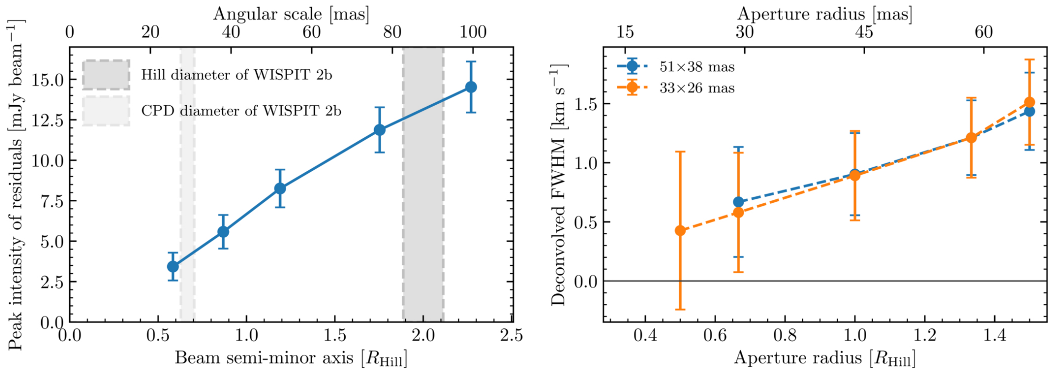
Figure 10. from Myriam Benisty et al 2026 Astrophys. J. Lett. 1009 doi:10.3847/2041-8213/aea214 https://dx.doi.org/10.3847/2041-8213/aea214 © 2026. The Author(s). Published by the American Astronomical Society.
