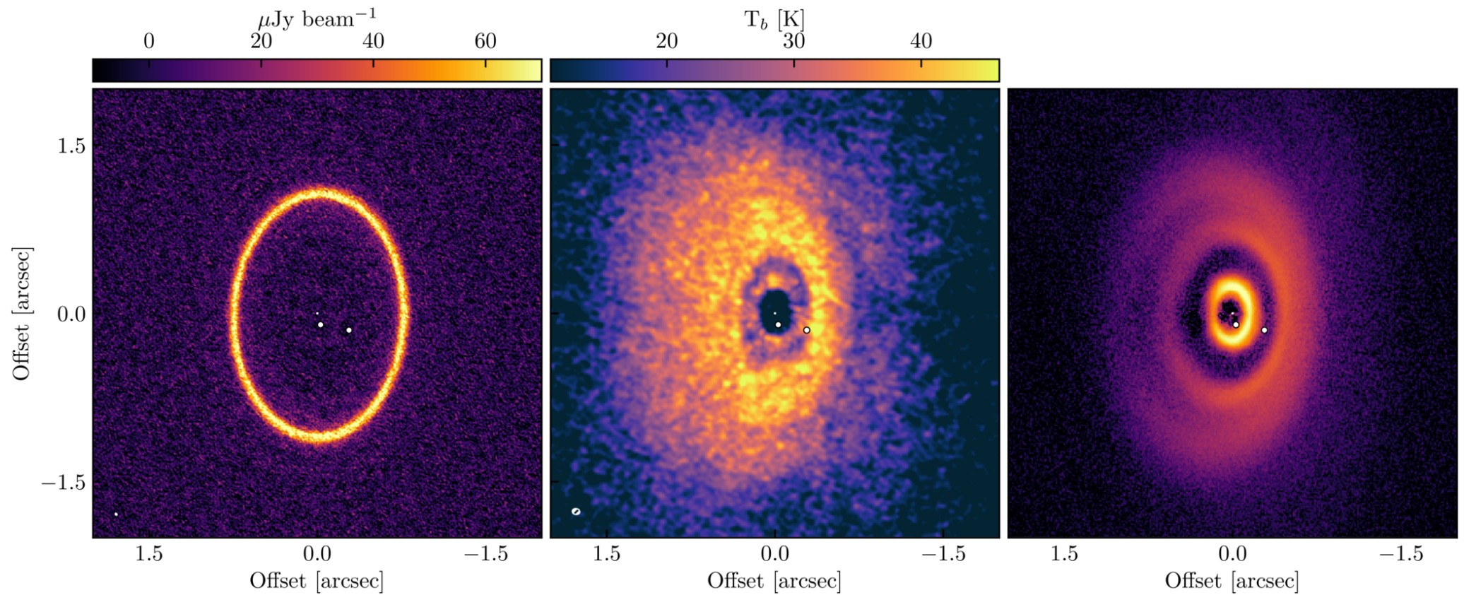
Figure 1. from Myriam Benisty et al 2026 Astrophys. J. Lett. 1009 doi:10.3847/2041-8213/aea214 https://dx.doi.org/10.3847/2041-8213/aea214 © 2026. The Author(s). Published by the American Astronomical Society.
