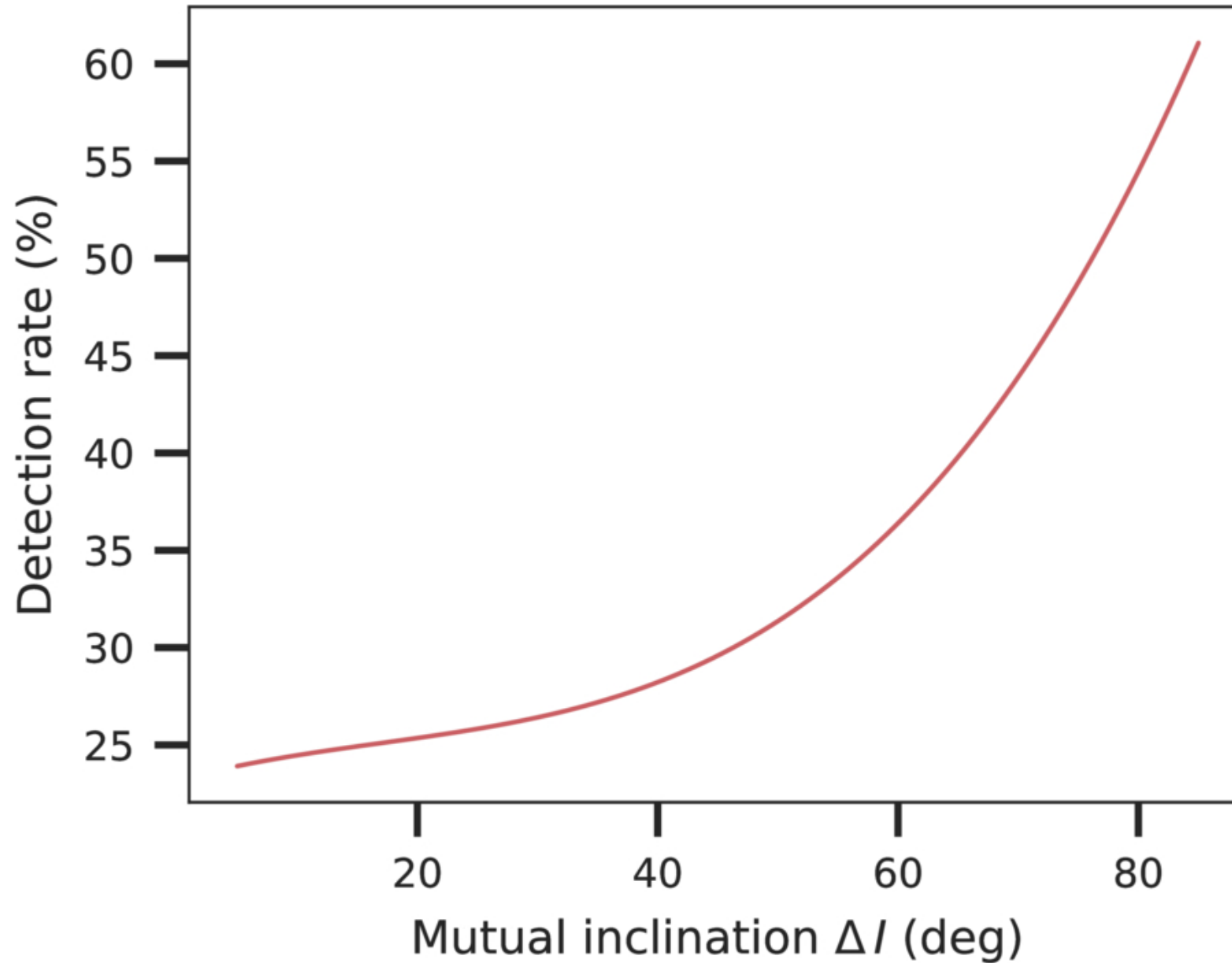
Figure G1. from Guang-Yao Xiao et al 2026 Astrophys. J. Lett. 1009 doi:10.3847/2041-8213/aea15e https://dx.doi.org/10.3847/2041-8213/aea15e © 2026. The Author(s). Published by the American Astronomical Society.
