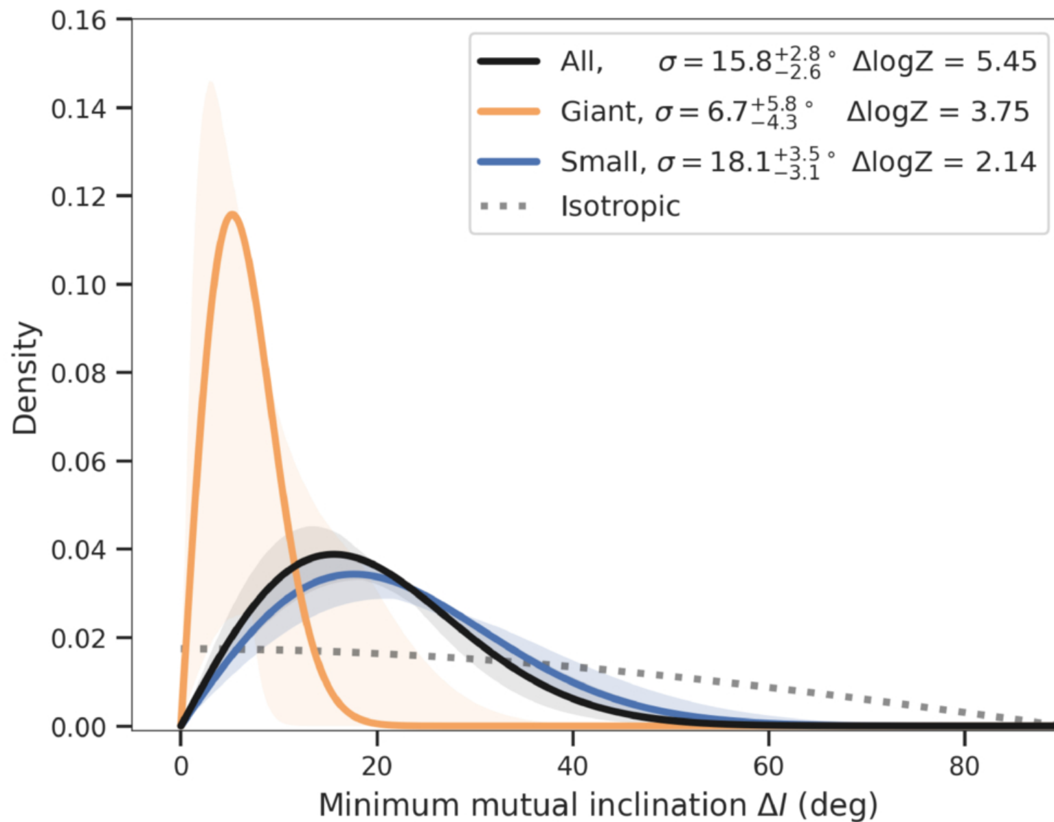
Figure 2. from Guang-Yao Xiao et al 2026 Astrophys. J. Lett. 1009 doi:10.3847/2041-8213/aea15e https://dx.doi.org/10.3847/2041-8213/aea15e © 2026. The Author(s). Published by the American Astronomical Society.
