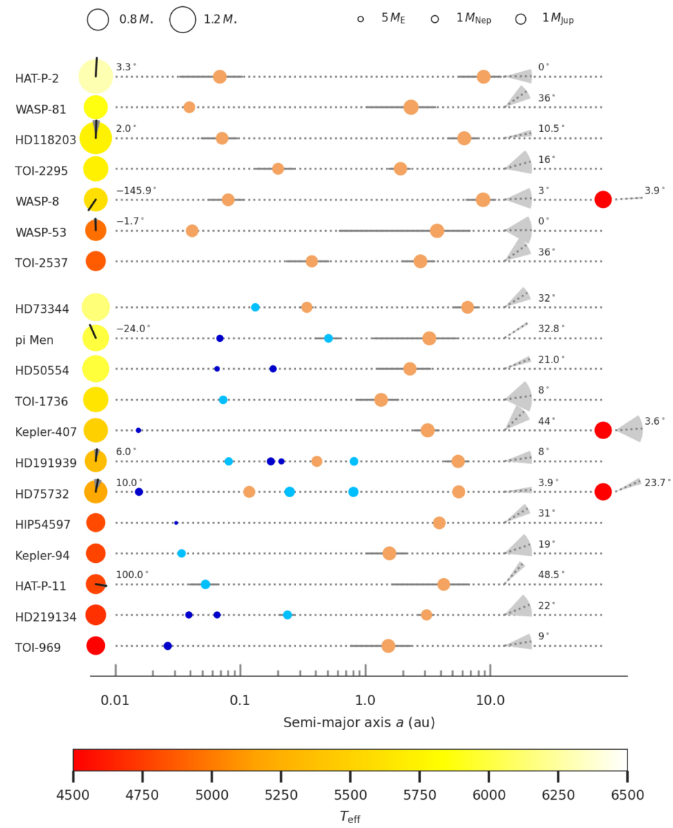
Figure 1. from Guang-Yao Xiao et al 2026 Astrophys. J. Lett. 1009 doi:10.3847/2041-8213/aea15e https://dx.doi.org/10.3847/2041-8213/aea15e © 2026. The Author(s). Published by the American Astronomical Society.
