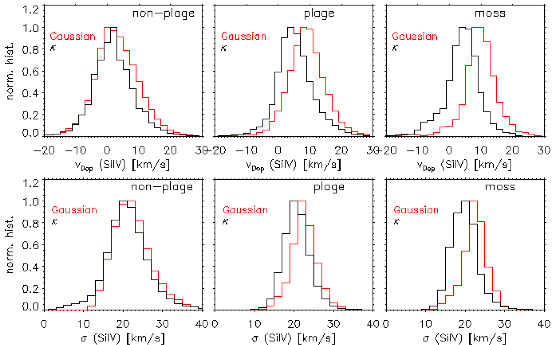
Figure 5. from Paola Testa et al 2026 Astrophys. J. Lett. 1009 doi:10.3847/2041-8213/aea155 https://dx.doi.org/10.3847/2041-8213/aea155 © 2026. The Author(s). Published by the American Astronomical Society.
