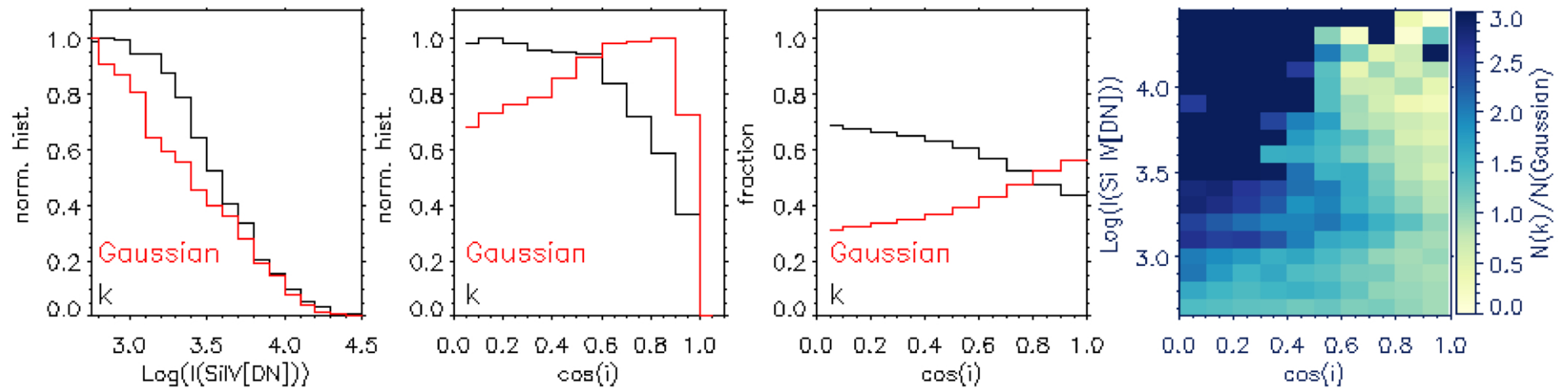
Figure 4. from Paola Testa et al 2026 Astrophys. J. Lett. 1009 doi:10.3847/2041-8213/aea155 https://dx.doi.org/10.3847/2041-8213/aea155 © 2026. The Author(s). Published by the American Astronomical Society.
