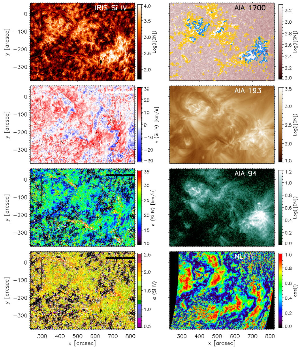
Figure 2. from Paola Testa et al 2026 Astrophys. J. Lett. 1009 doi:10.3847/2041-8213/aea155 https://dx.doi.org/10.3847/2041-8213/aea155 © 2026. The Author(s). Published by the American Astronomical Society.
