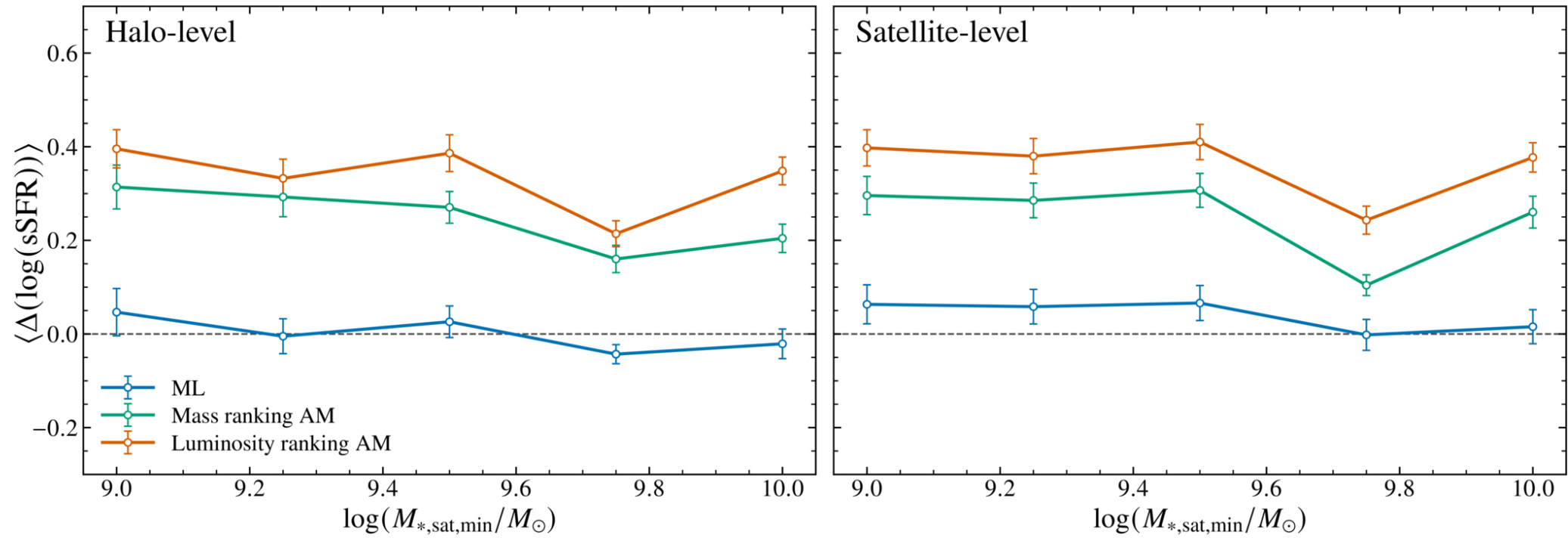
Figure 3. from Dingyi Zhao et al 2026 Astrophys. J. Lett. 1009 doi:10.3847/2041-8213/aea142 https://dx.doi.org/10.3847/2041-8213/aea142 © 2026. The Author(s). Published by the American Astronomical Society.
