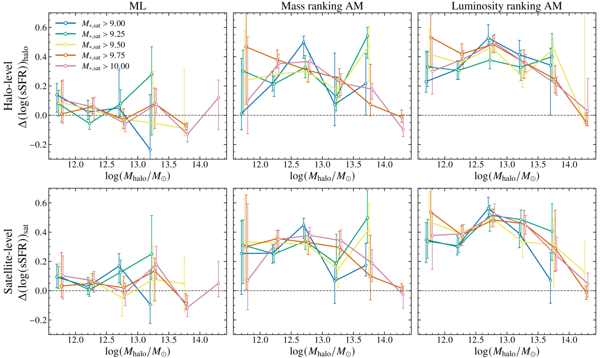
Figure 2. from Dingyi Zhao et al 2026 Astrophys. J. Lett. 1009 doi:10.3847/2041-8213/aea142 https://dx.doi.org/10.3847/2041-8213/aea142 © 2026. The Author(s). Published by the American Astronomical Society.
