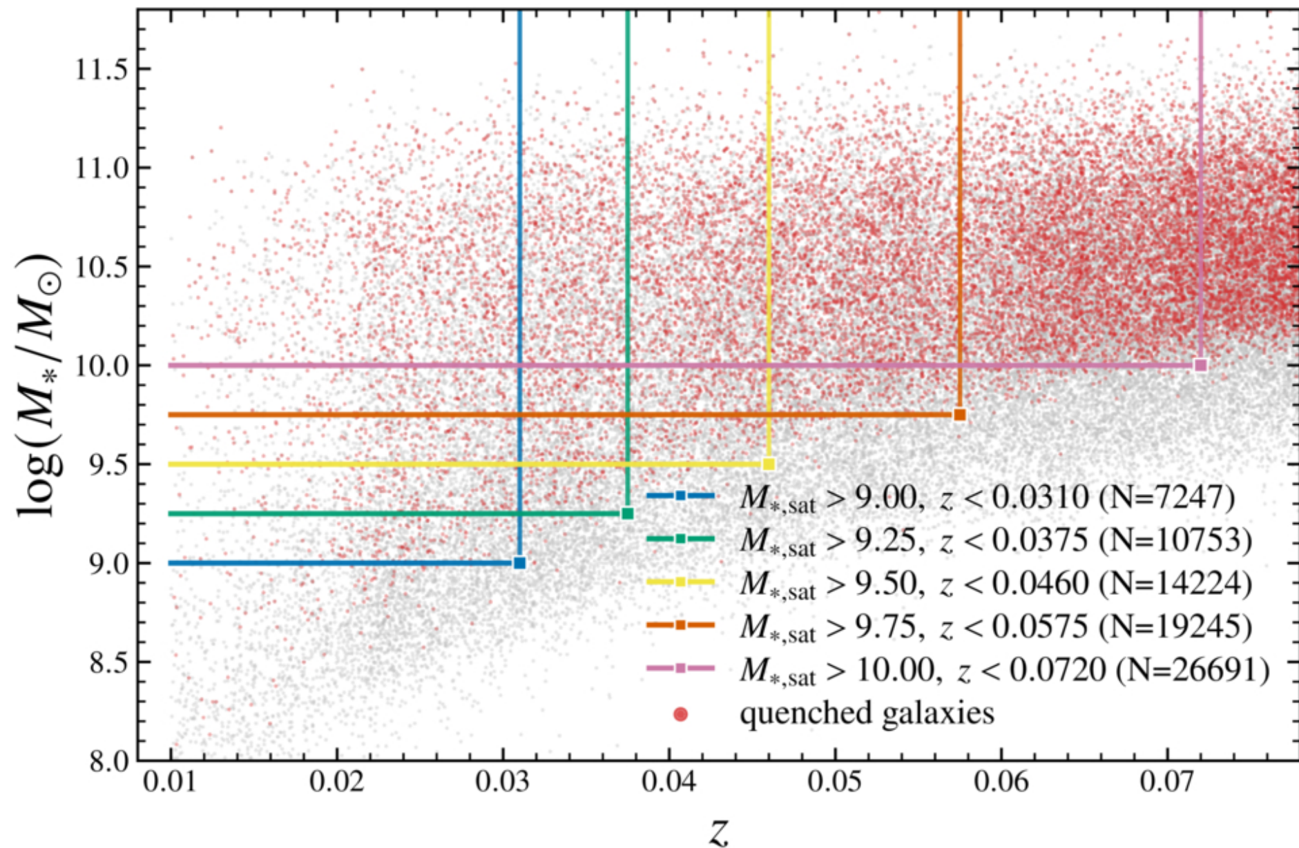
Figure 1. from Dingyi Zhao et al 2026 Astrophys. J. Lett. 1009 doi:10.3847/2041-8213/aea142 https://dx.doi.org/10.3847/2041-8213/aea142 © 2026. The Author(s). Published by the American Astronomical Society.
