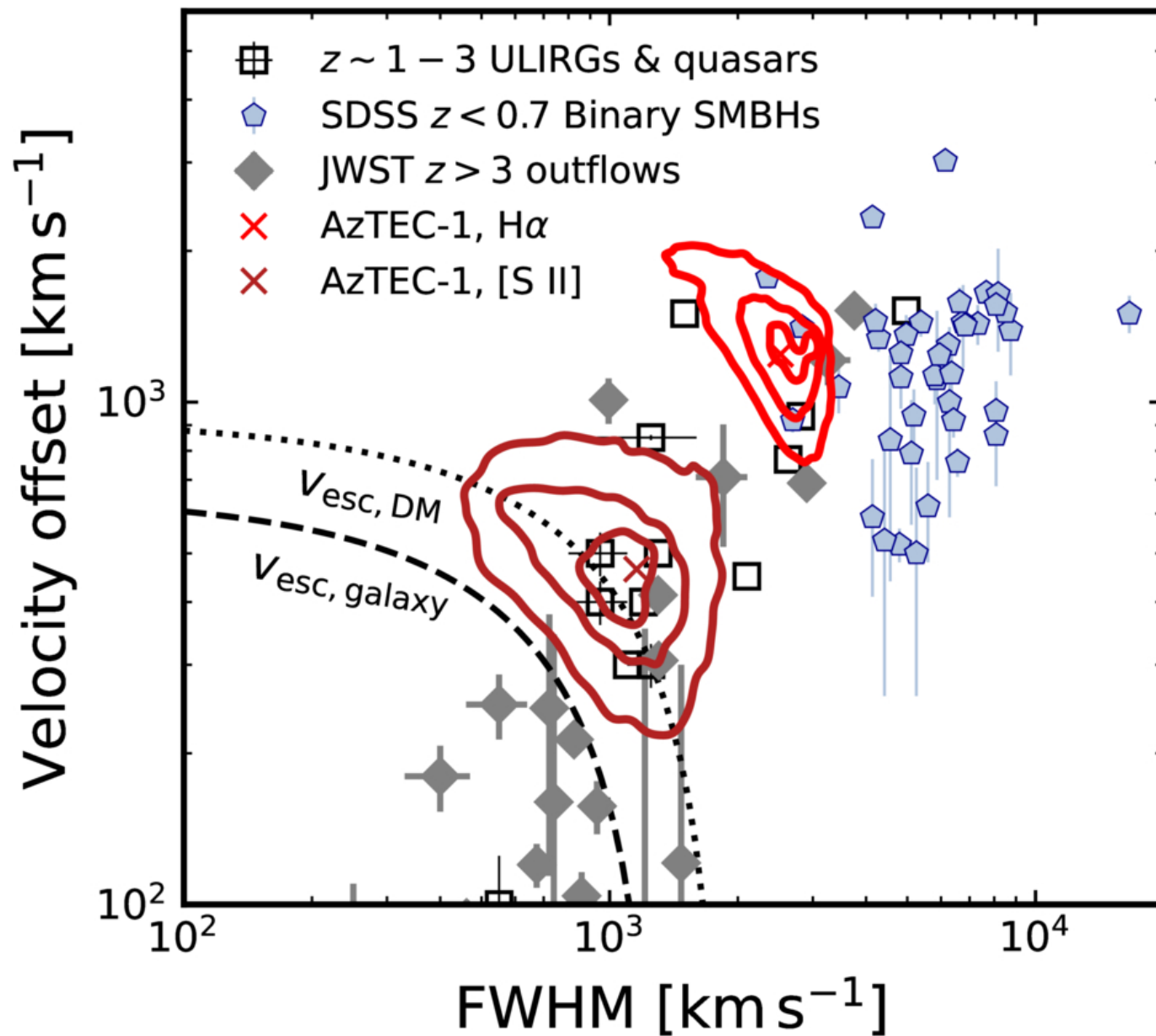
Figure 9. from Jed McKinney et al 2026 Astrophys. J. Lett. 1011 doi:10.3847/2041-8213/aea0cd https://dx.doi.org/10.3847/2041-8213/aea0cd © 2026. The Author(s). Published by the American Astronomical Society.
